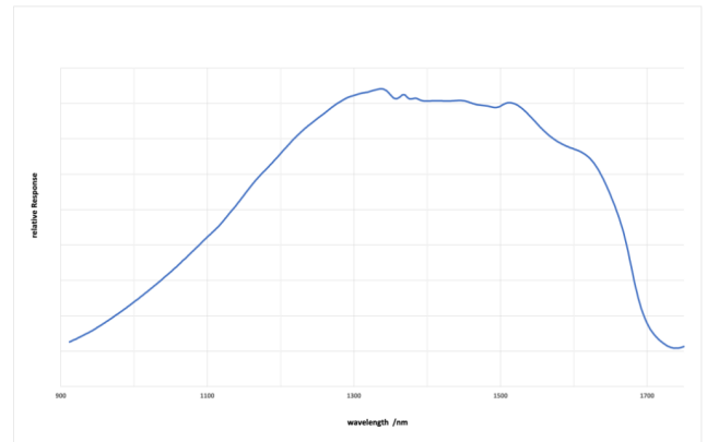
BlackIndustry SWIR 1.7 - Spectral response
